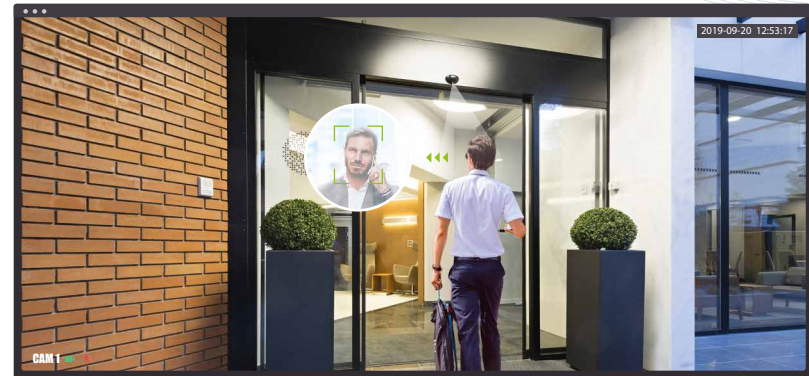
Face Detection
