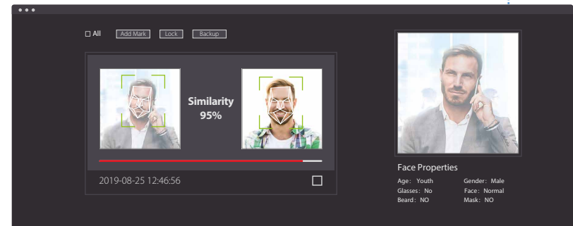
Similarity Comparison
